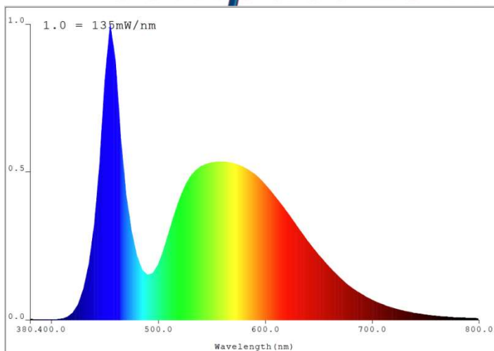
Distribution Curve of Meridian
